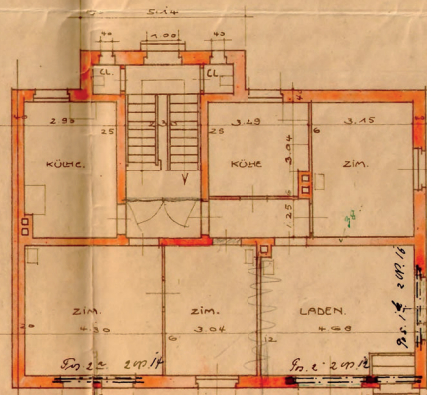
ERDGESHOSS.
