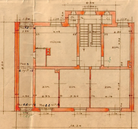
ERDGESCHOSS.
